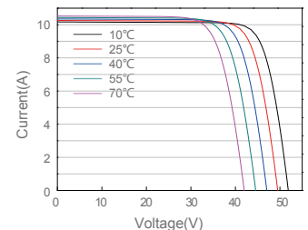
Current-Voltage Curve
